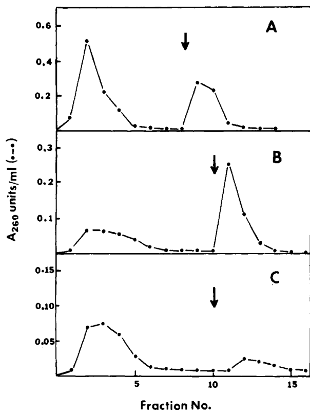
FIGURE 1: Chromatography of chemically misacylated E. coli N -acetyl-DL-β-phenylalanyl-tRNA Phe on DEAE-cellulose (panel A), on BD-cellulose (panel B), and on BD-cellulose after alkali treatment (panel C). E. coli tRNA Phe -C OH (9; 0.6 A 260 unit) was incubated with pCpA-DL-β-phenylalanyl-tRNA Phe (8f; 0.3 A 260 unit) in a reaction volume (70 μL) containing 55 mM Na + -Hepes, pH 7.5, 15 mM MgCl 2 , 250 μM ATP, 20 μg/mL bovine serum albumin, 10% dimethyl sulfoxide, and 24 units of T4 RNA ligase. The reaction mixture was incubated at 4 °C for 16 h and then diluted to 0.5 mL with 50 mM NaOAc, pH 4.5, containing 10 mM MgCl 2 . The sample was applied to a 1.0-mL DEAE-cellulose column (4 °C) that had been equilibrated in the same buffer, and the column was washed with (eight 1.0-mL fractions of) 50 mM NaOAc, pH 4.5, containing 10 mM MgCl 2 and 0.25 M NaCl to remove RNA ligase and other non-tRNA reaction components. Elution of tRNAs 9 and 10 was then effected with five 1.0-mL fractions of the same buffer containing 1.0 M NaCl (panel A). The tRNA-containing fractions were pooled and applied to a 1.0-mL BD-cellulose column (4 °C) that had been equilibrated with 50 mM NaOAc, pH 4.5, containing 10 mM MgCl 2 and 1.0 M NaCl. Unreacted tRNA Phe -C OH (9) was removed by washing the column with 10 mL of the same buffer; the column was then eluted with the same buffer containing 25% ethanol to effect elution of N -acetyl-DL-β-phenylalanyl-tRNA Phe (panel B). Fractions 11 and 12 were pooled, dialyzed against 1 mM NaOAc, pH 4.5, and concentrated to a small volume. The isolated yield of N -acetyl-DL-β-phenylalanyl-tRNA Phe was 0.34 A 260 unit (57%). N -Acetyl-DL-β-phenylalanyl-tRNA Phe (0.25 A 260 unit) was treated with 0.5 mL of 50 mM Tris-HCl, pH 9.5, containing 10 mM MgCl 2 at 4 °C for 16 h, and then diluted with 1 mL of 50 mM NaOAc, pH 4.5, containing 10 mM MgCl 2 and 1.0 M NaCl, and again subjected to chromatography on BD-cellulose (panel C). The elution conditions were identical with those described for panel B.
